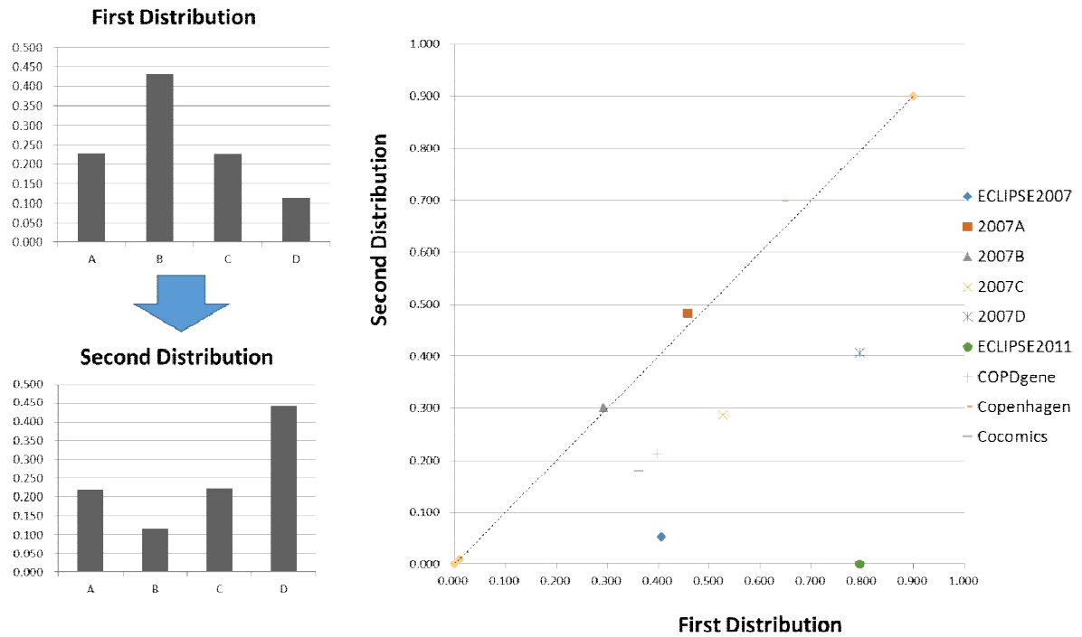
Fig.1. Similarities among the A-B-C-D categories in the cohorts including sub-cohorts A, B, and C in ECLIPSE 2007 as well as COPDgene, Copenhagen, and Cocomics.
